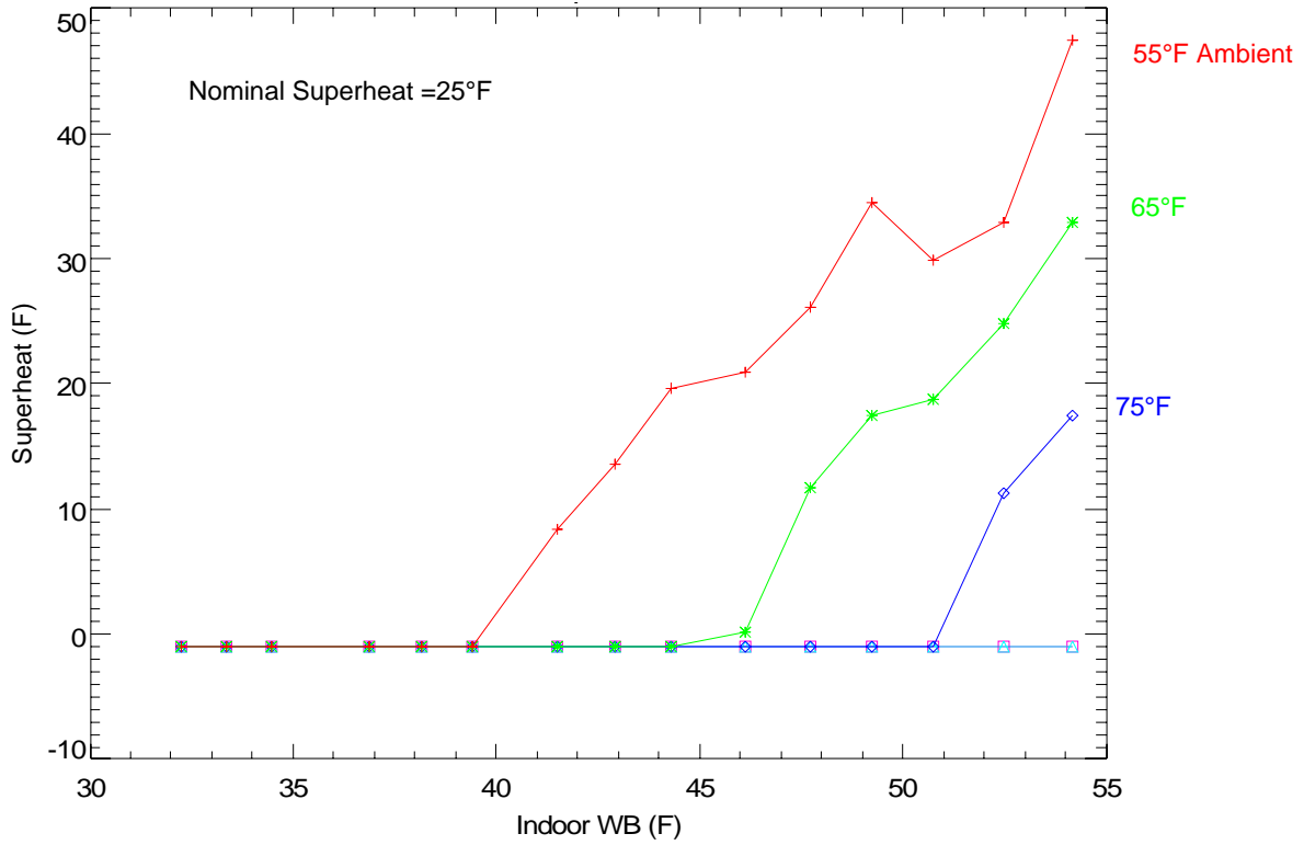
Figure C-6. Compressor Superheat at COOLBOT Operating Conditions (WB)
